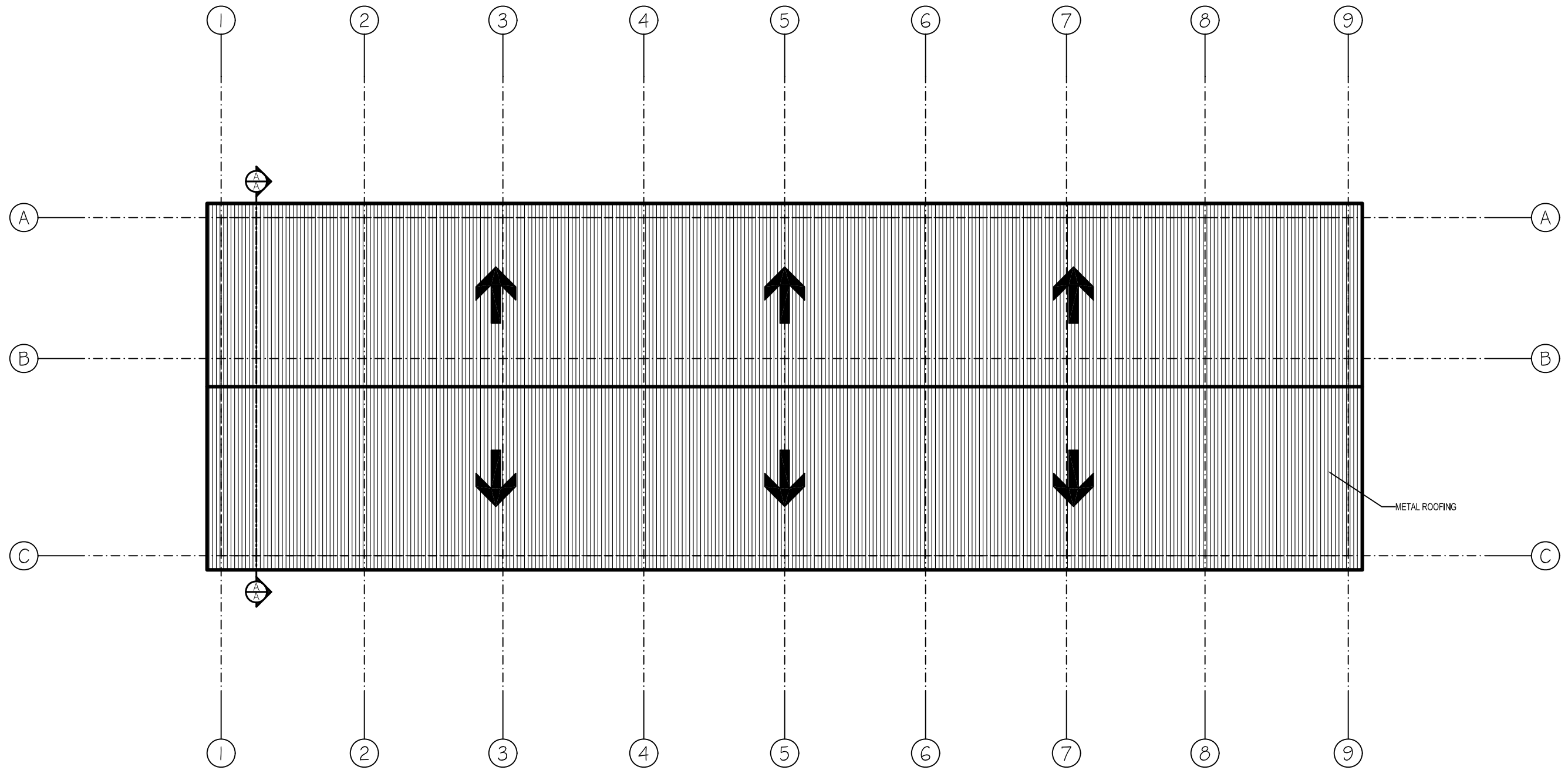
ROOF PLAN PG. 8 OF 16 SCALE: 1/8" = 1'-0"
